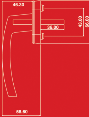
3100 İnci Plastik Pencere Kolu (demirli) İnci Plastic Window Handle (with iron support)
